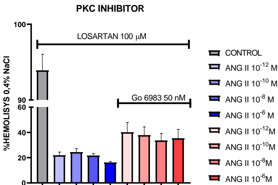
Fig. 8. Osmotic fragility of red blood cells in NaCl 0.4% treated with GO 6983 (50 nM) plus Angiotensin II (10 -6 M, 10 -8 M, 10 -10 M, 10 -12 M) and losartan. No significant results were obtained when adding Go 6983 compared with only angiotensin II and losartan, therefore no protection against hemolysis occurs through this pathway. The blue bars represent Ang II plus losartan and the red bars had the addition of GO 6983. N=3 in triplicate. Values are mean ±SEM. * = p <0.05, ** = p <0.01, *** = p <0.001 and **** = p < 0.0001 vs same concentration without GO 6983; with a 95% confidence interval in One-way ANOVA and Tukey post-test.
