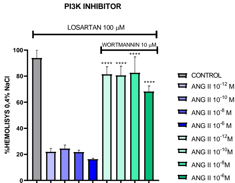
Fig. 5. Osmotic fragility of red blood cells in NaCl 0.4% treated with Wortmannin (10 μM) plus Angiotensin II (10 -6 M, 10 -8 M, 10 -10 M, 10 -12 M) and losartan (100 μM). Wortmannin reversed the effect of Angiotensin II plus losartan in all four concentrations protecting erythrocyte from hemolysis. The blue bars represent Ang II plus losartan and the green bars had the addition of Wortmannin. N=3 in triplicate. Values are mean ±SEM. * = p < 0.05, ** = p < 0.01, *** = p < 0.001 and **** = p < 0.0001 vs same concentration without Wortmannin; with a 95% confidence interval in One-way ANOVA and Tukey post-test.
