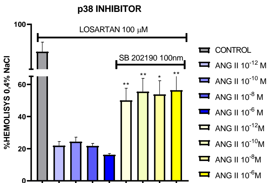
Fig. 7. Osmotic fragility of red blood cells in NaCl 0.4% treated with SB 202190 (100 nM) plus Angiotensin II (10 -6 M, 10 -8 M, 10 -10 M, 10 -12 M) and losartan. SB 202190 reversed the effect of Angiotensin II (10 -6 M, 10 -8 M, 10 -10 M, 10 -12 M) plus losartan, demonstrating a decrease of hemolysis in all four concentrations. The blue bars represent Ang II plus losartan and the yellow bars had the addition of SB 202190 N=3 in triplicate. Values are mean ±SEM. * = p <0.05, ** = p <0.01, *** = p <0.001 and **** = p < 0.0001 vs same concentration without SB 202190; with a 95% confidence interval in One-way ANOVA and Tukey post-test.
